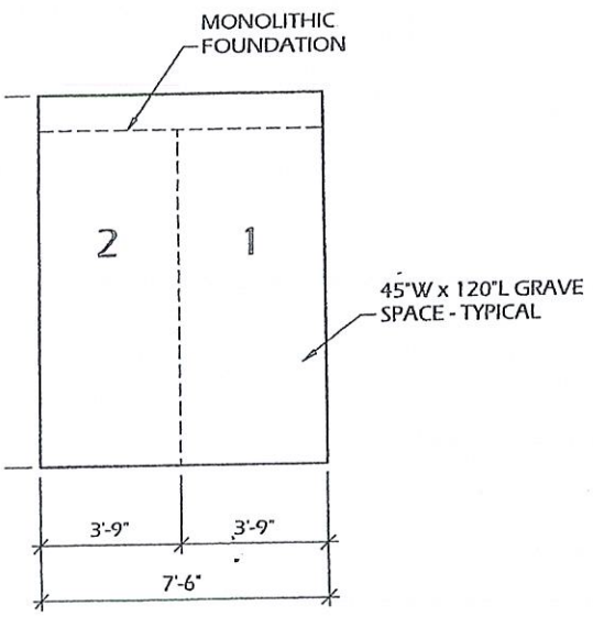
TYPICAL LOT WITH MONOLITH Scale 3/16" = 1'-0"
